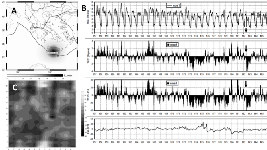
Figure 3. OLR and GPS/TEC analysis for M6.4 of 08.06.08. A. OLR anomaly from 06.08.08(07.30LT). B. GPS/TEC time series (05.15.08-06.14.08); C. Map of 3-D pattern of \Delta TEC for M6.4 of 06.08.08;
