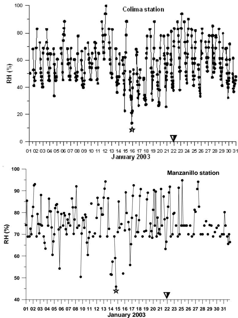
Fig. 2. Top panel: Relative humidity at Colima station for January 2003. Bottom panel: The same at Manzanillo station. \nabla indicates the earthquake moment, stars indicate the parameters peculiarities, interpreted as precursor phenomena.
